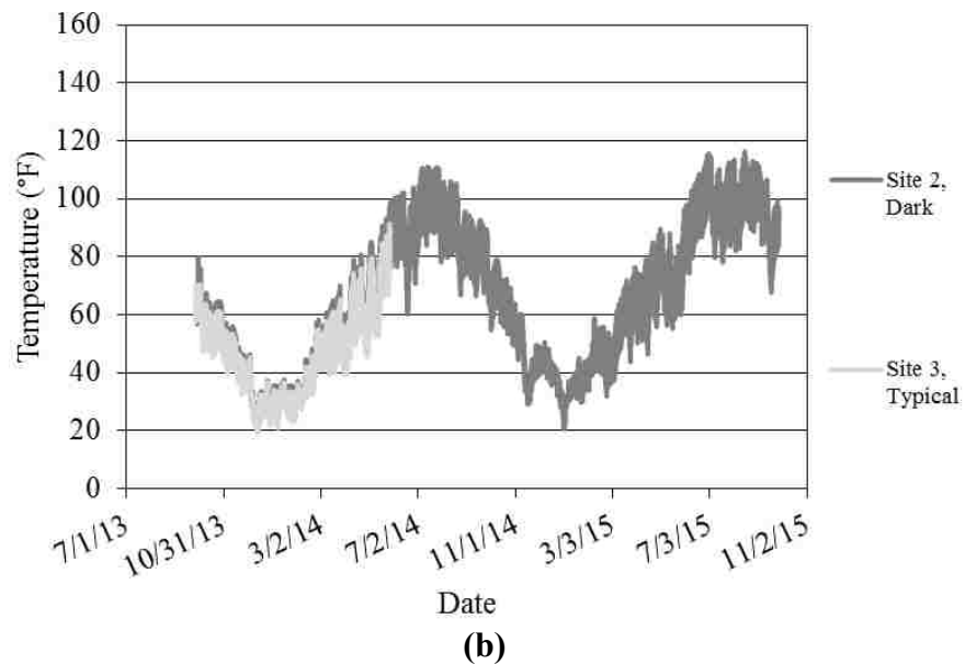
Figure A-25: Lower pavement temperature for (a) site 1 and (b) sites 2 and 3.
