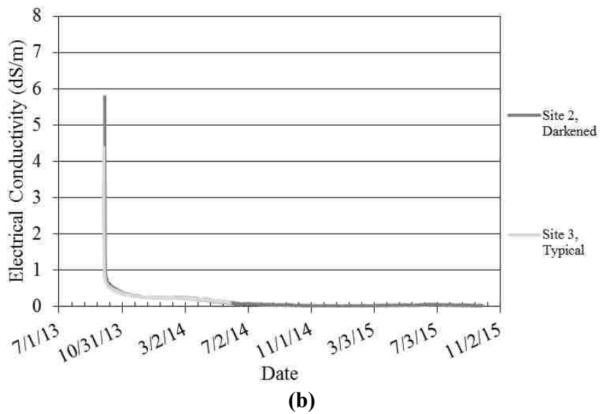
Figure A-29: Lower pavement electrical conductivity for (a) site 1 and (b) sites 2 and 3
