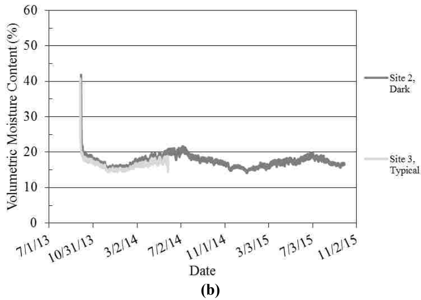
Figure A-27: Lower pavement moisture for (a) site 1 and (b) sites 2 and 3.
