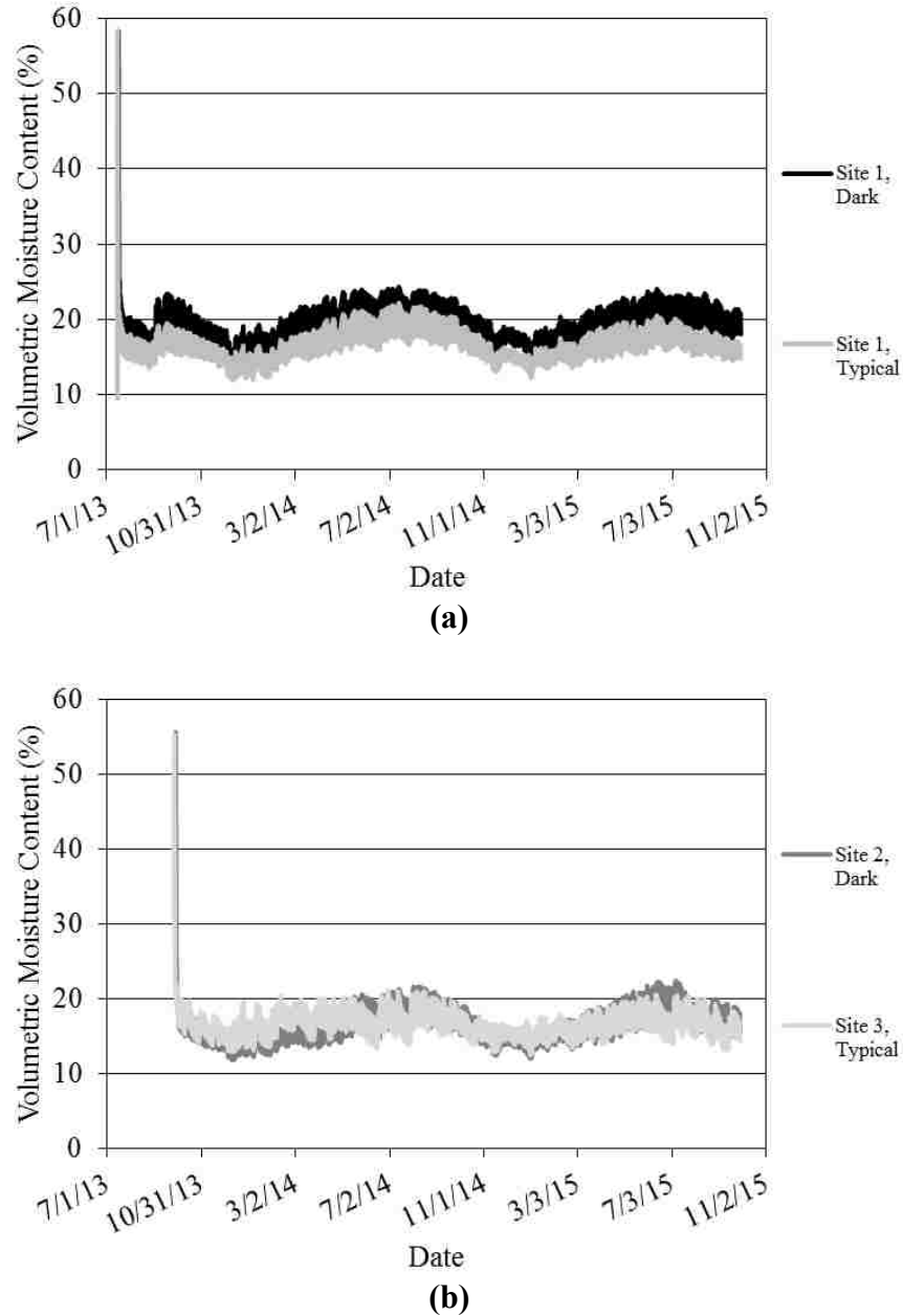
Figure A-26: Upper pavement moisture for (a) site 1 and (b) sites 2 and 3.
